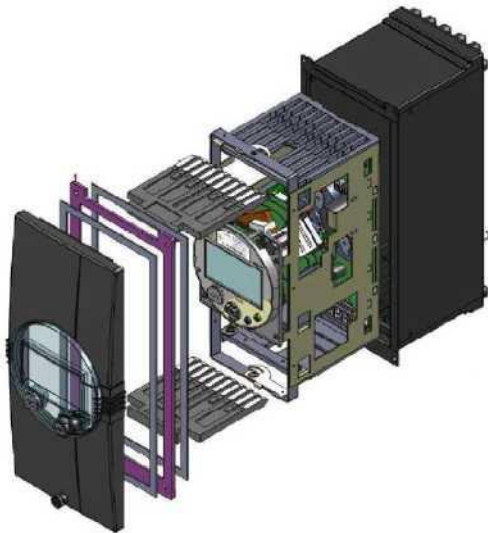
Example of a JEMStar II retrofitting a JEM2 using an existing 'tall' meter enclosure.
